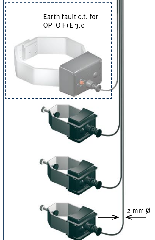
Add-on housing
