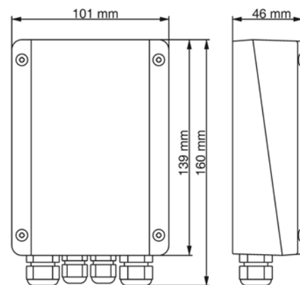
Add-on housing
