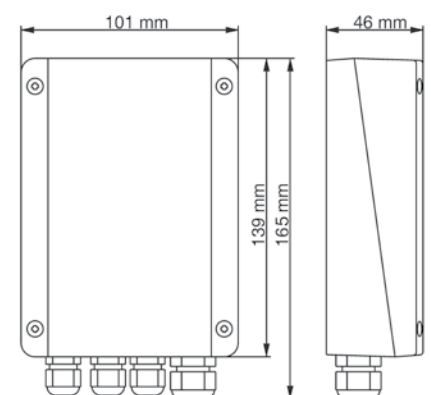
Add-on housing
