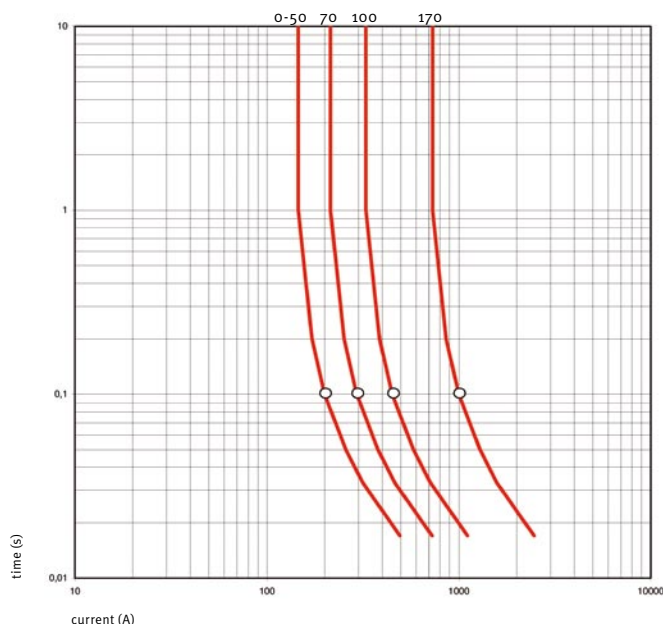
Time /current characteristic Navigator LM
