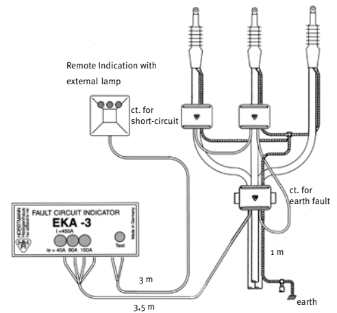
Mounting, schematical
